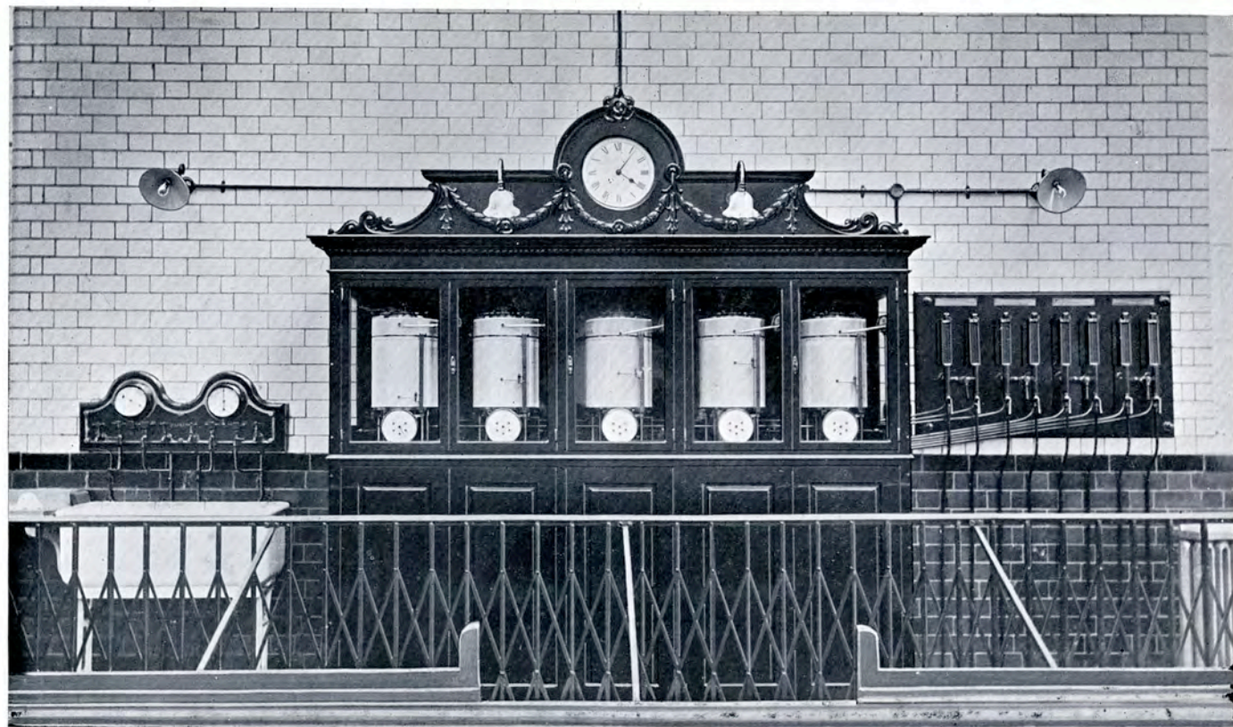
Sample Basin and Venturi Meter Recorders (Brushes Filter House)
