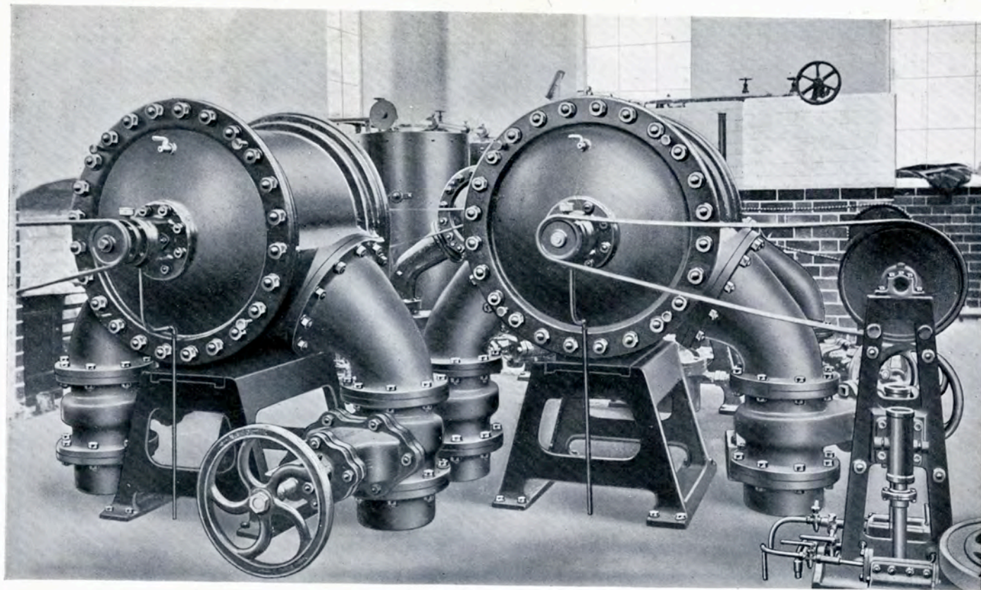
Water Motors, Chemical Pumps, Lime and Alumina Tanks (Brushes Filter House)
