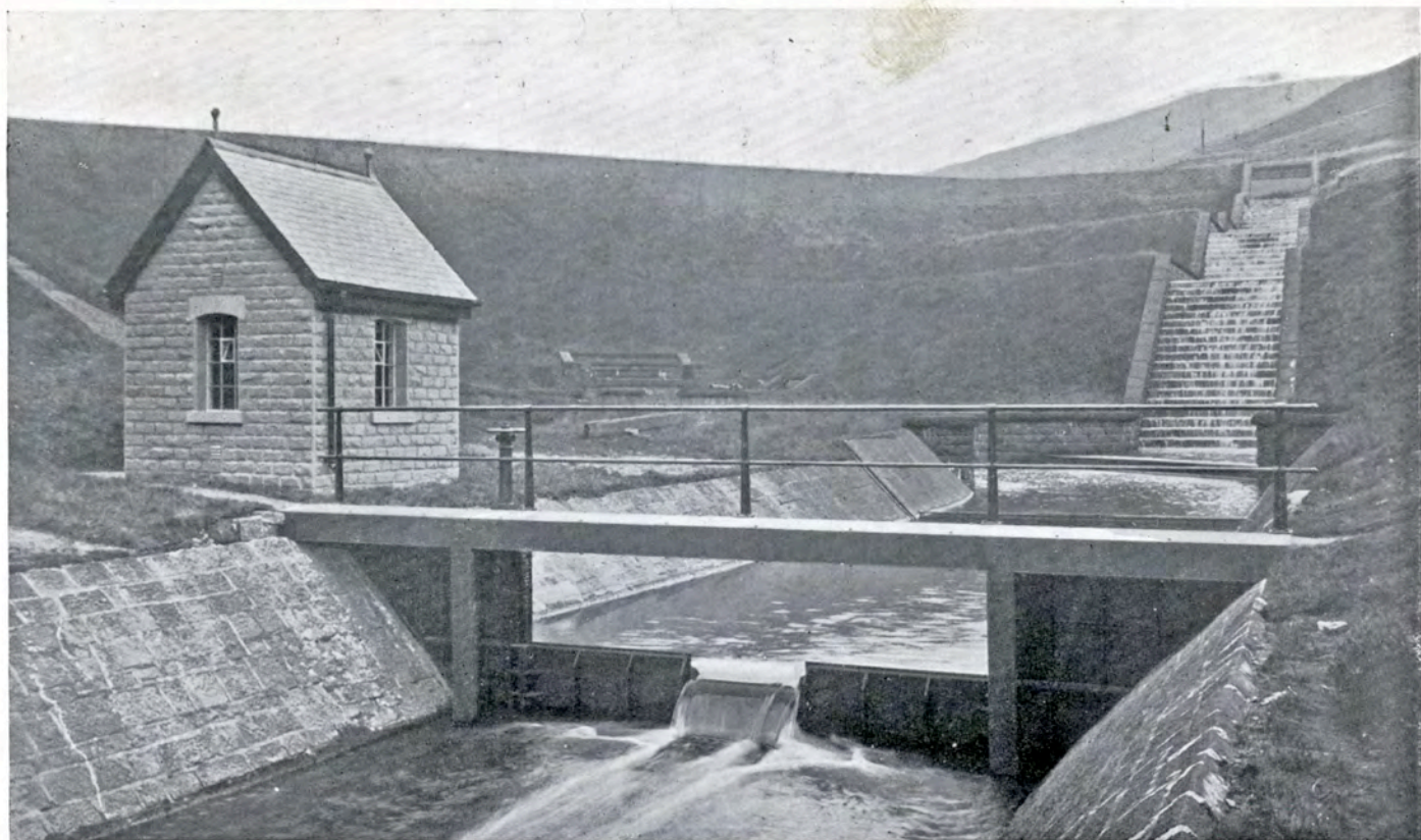
Compensation Water Weir Gauge Recorder (Yeoman Hey Reservoir Water Course)
